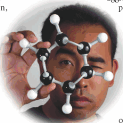
Benzene, whose molecular structure is depicted in this model, is considered the first highly publicized chemical carcinogen in the age of OSHA.
